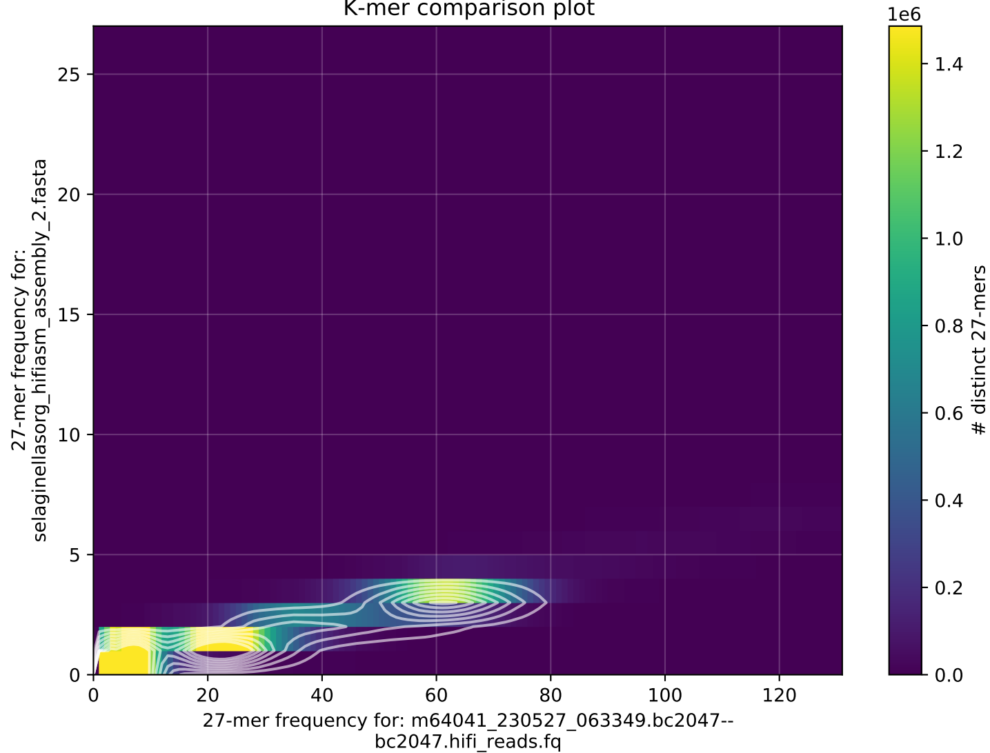
K-mer comparison plot
