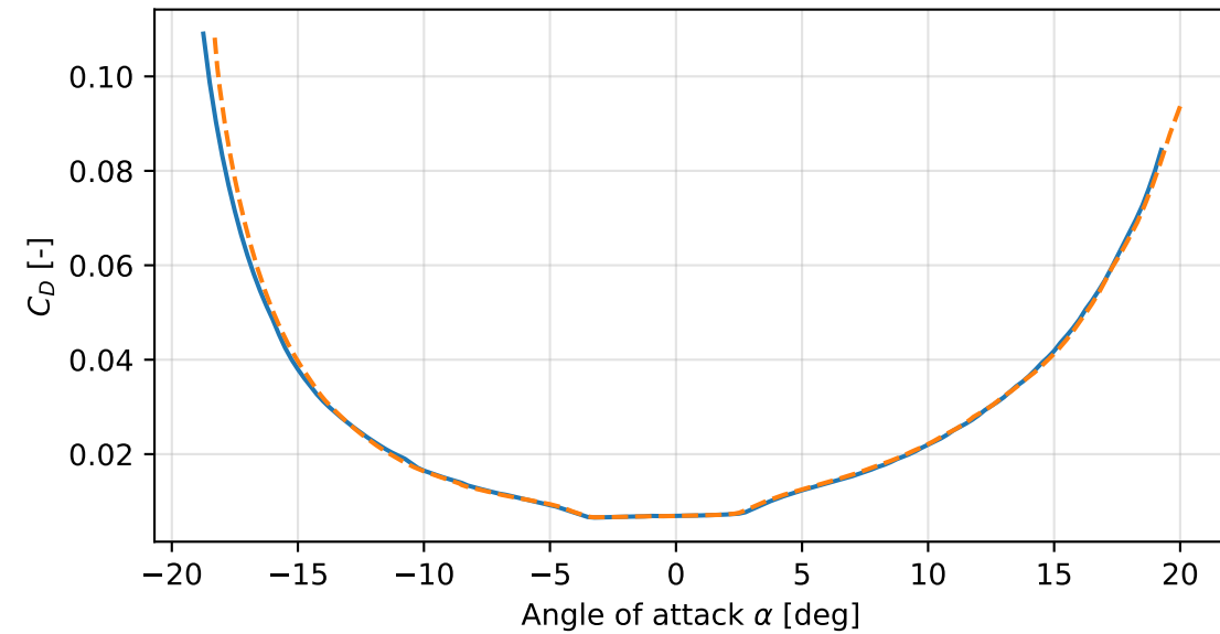
Drag curve
