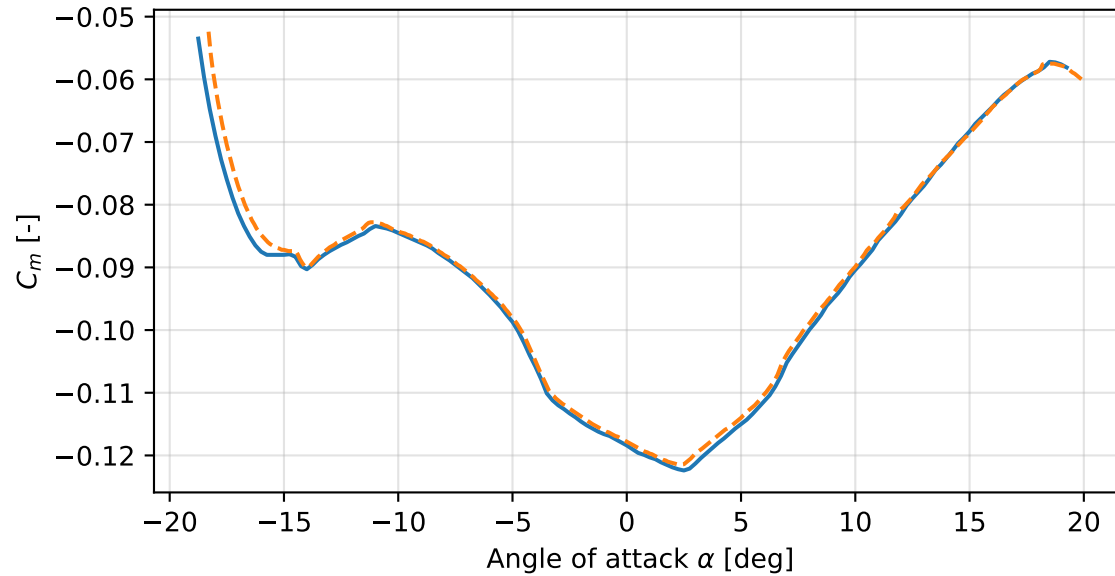
Moment curve
