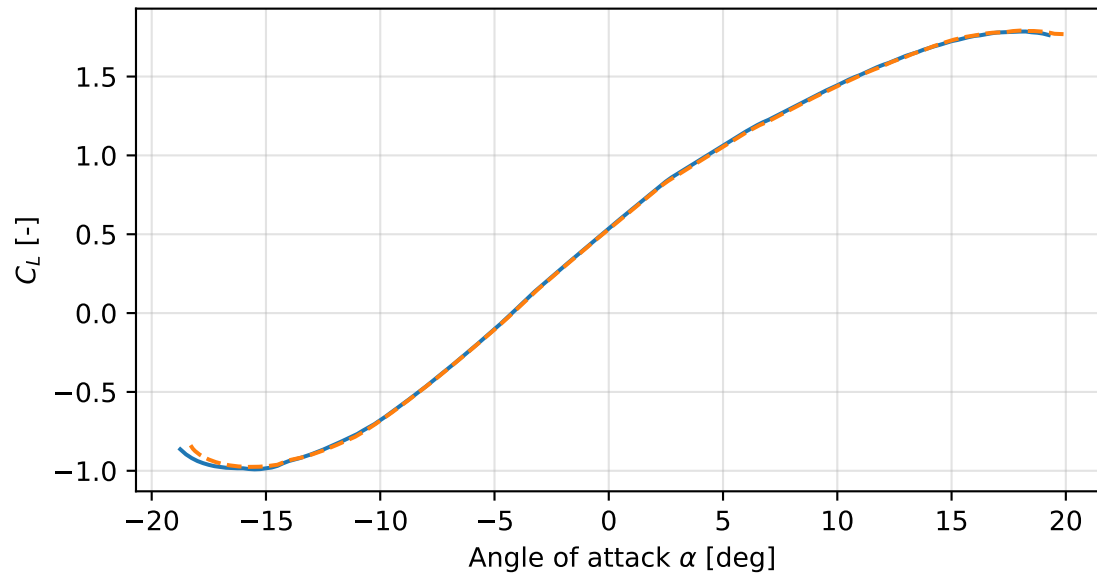
Lift curve
