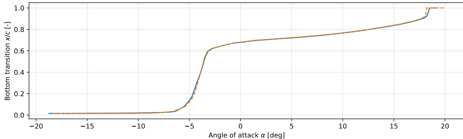
Lower-surface transition
