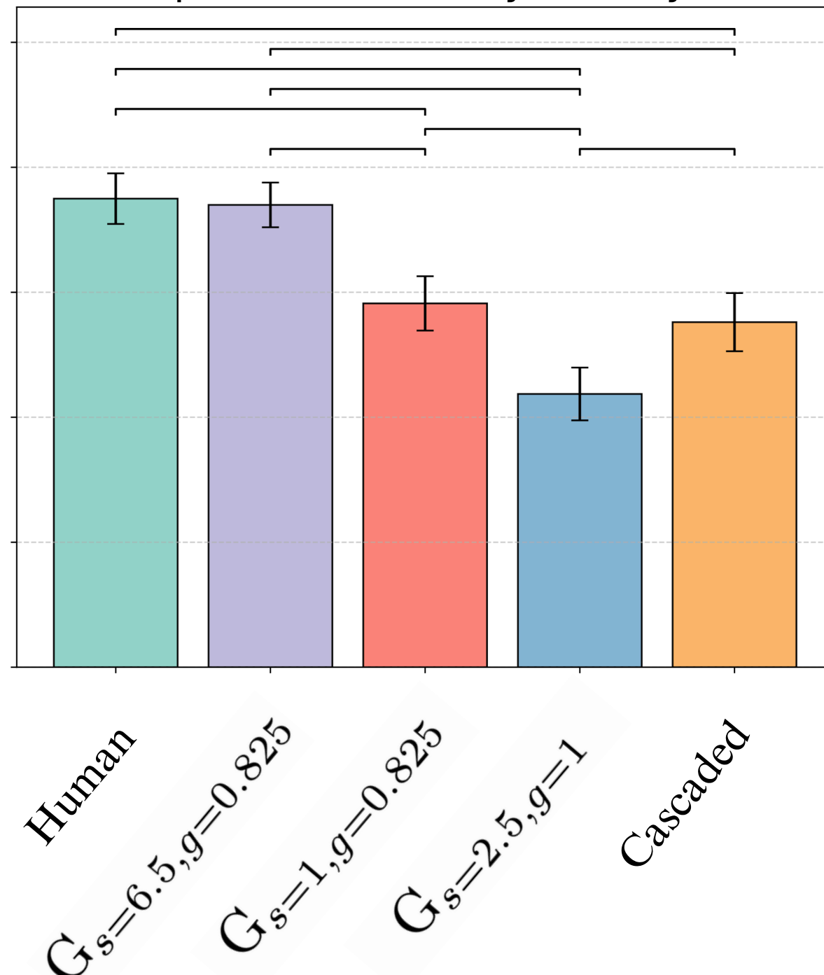
Speech-Gesture Synchrony
