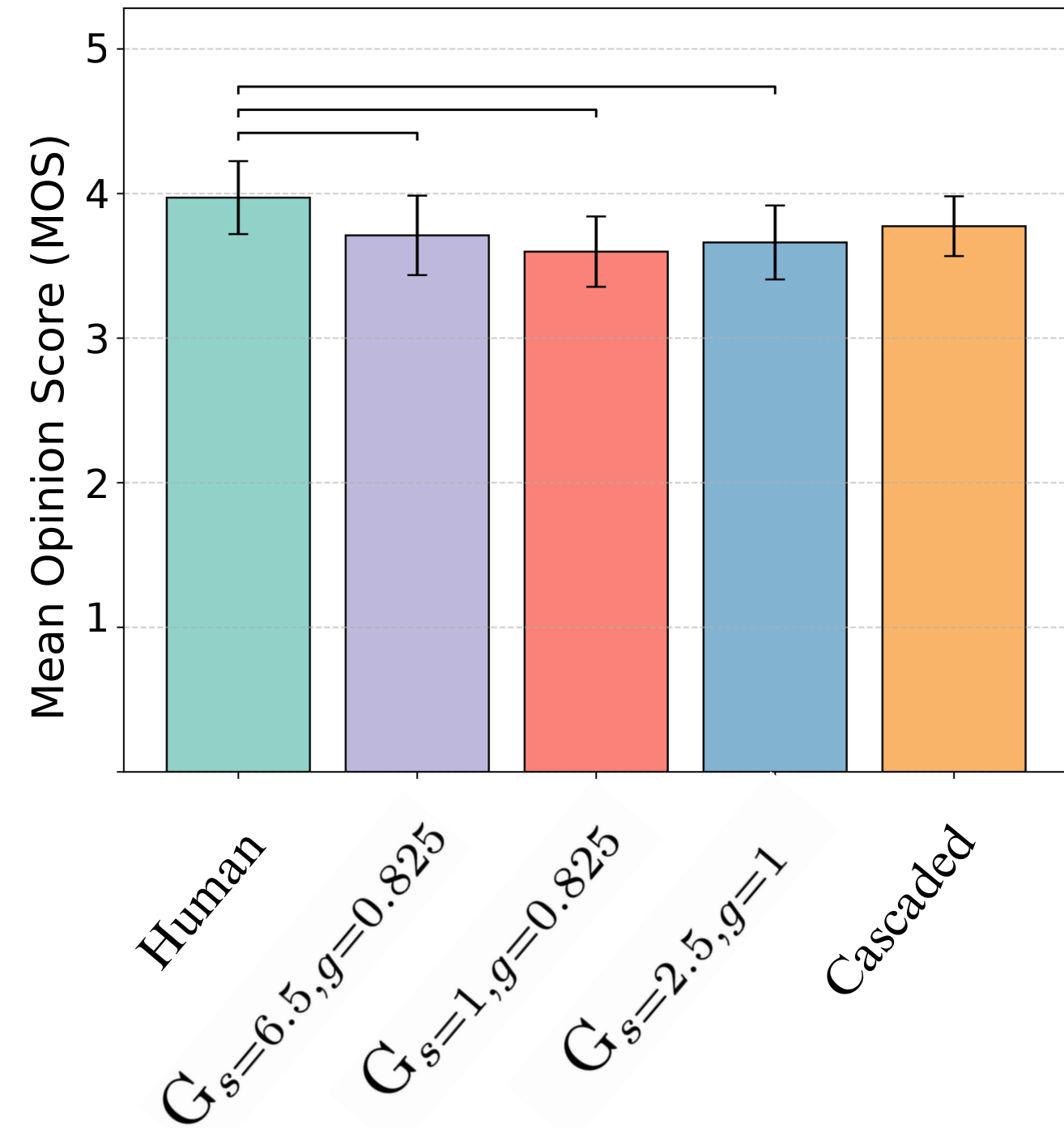
Voice Human-likeness
