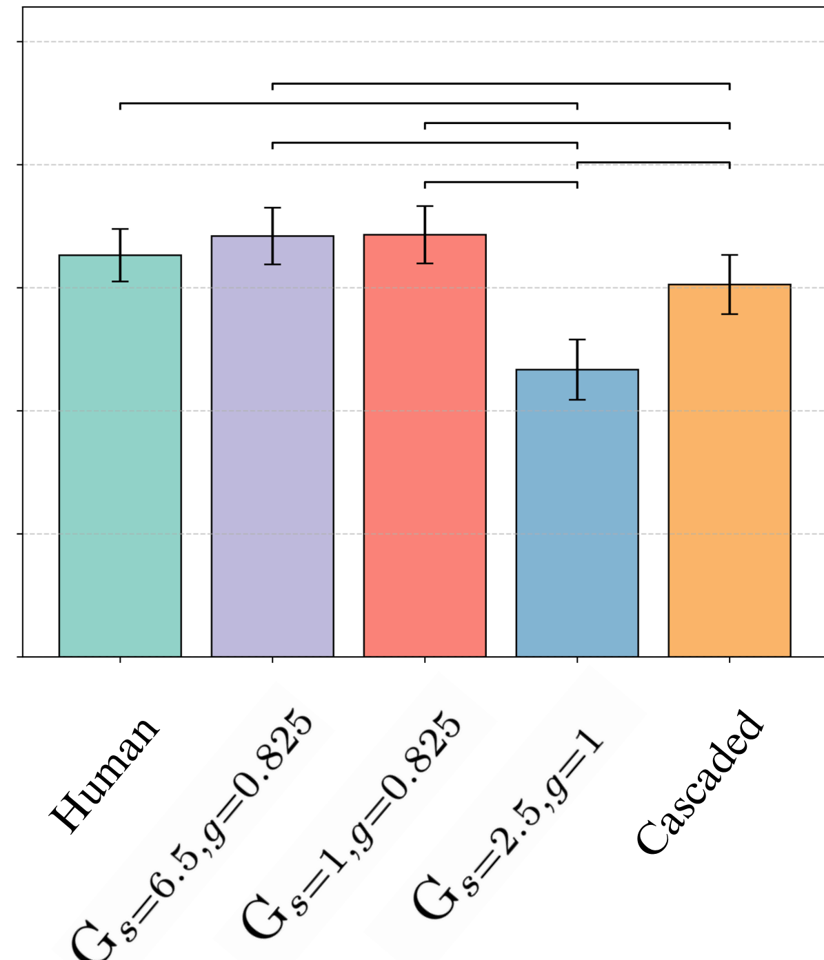
Gesture Human-likeness
