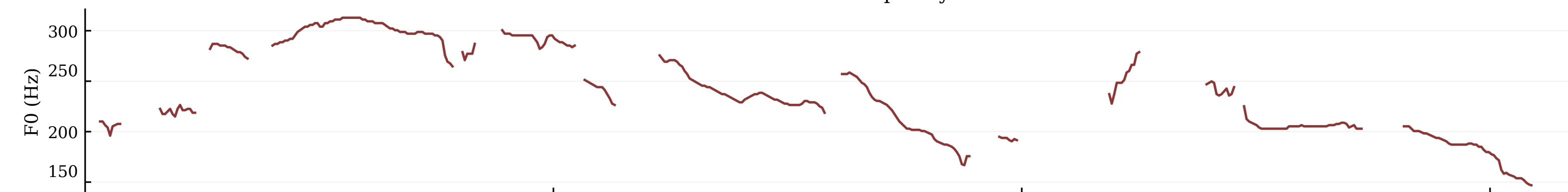
Fundamental frequency
