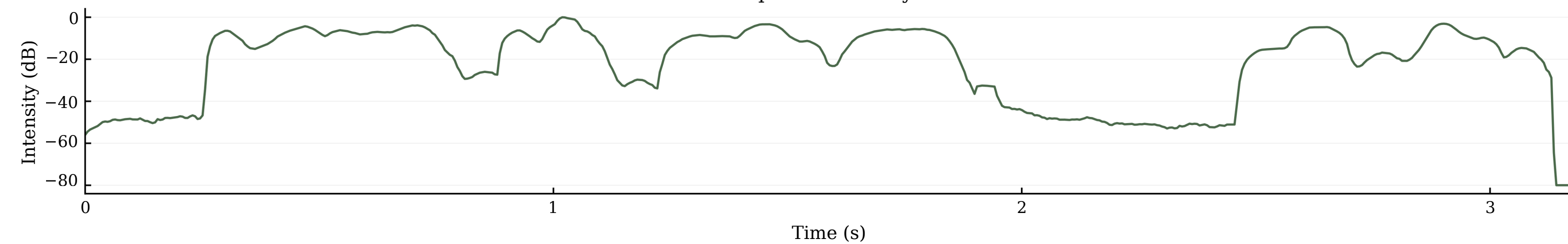
Speech intensity
