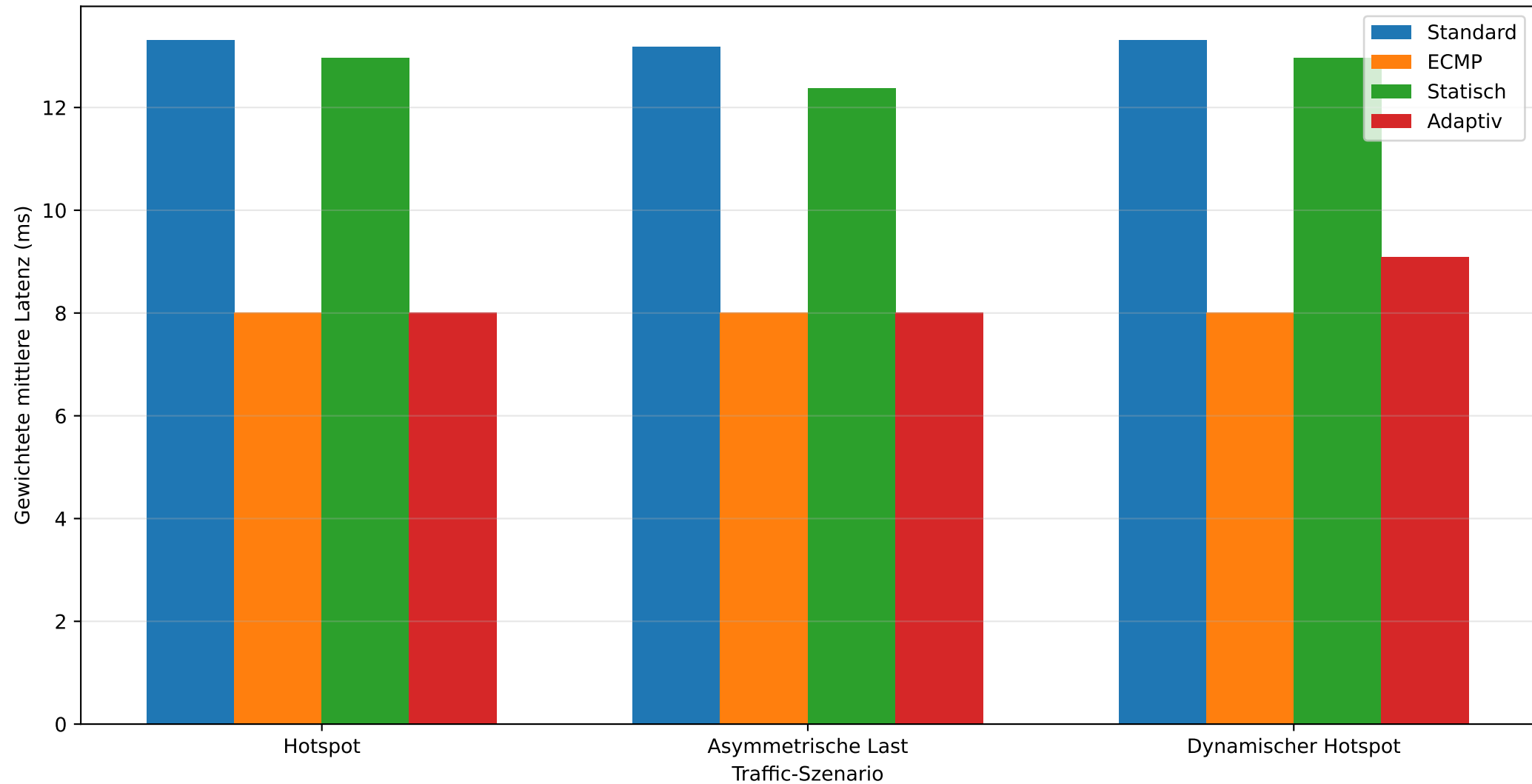
Mittlere Latenz - Traffic-Engineering-Szenarien
