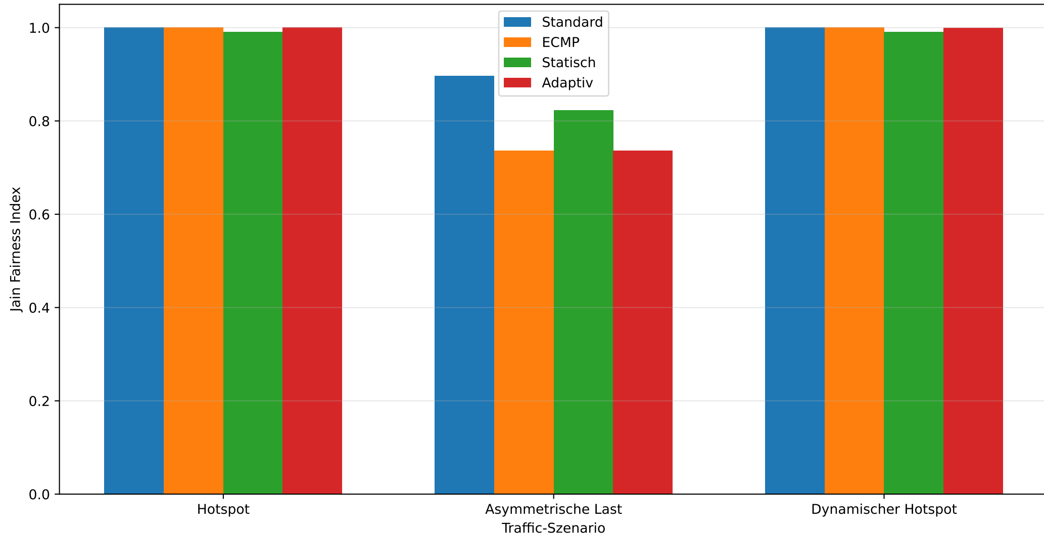
Fairness - Traffic-Engineering-Szenarien
