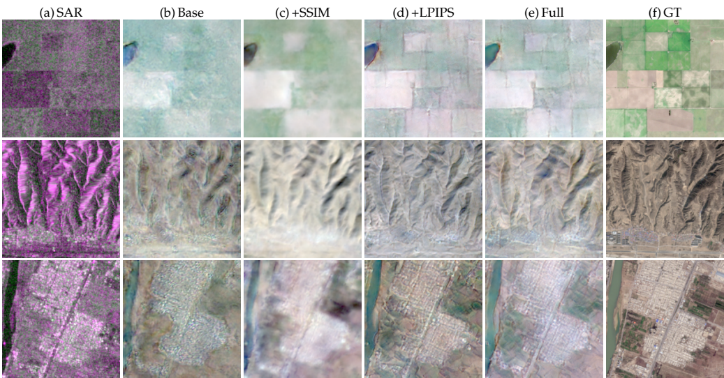
Figure 5. Visual comparison of loss configurations. (a) Input SAR, (b) Baseline ( \mathcal{L}_{\text{GAN}}+\mathcal{L}_{\text{L1}} ), (c) Baseline w/ SSIM, (d) Baseline w/ LPIPS, (e) Proposed full loss, (f) Ground Truth.
