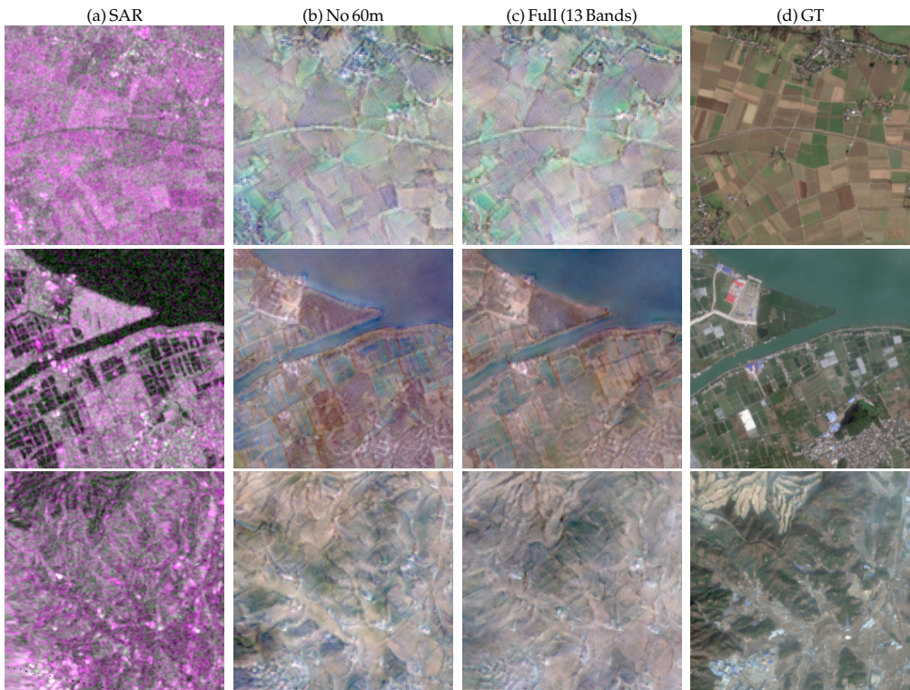
Figure 8. Qualitative results comparing models trained with and without the 60 m bands. (a) SAR input, (b) 10-band model output, (c) 13-band model output, (d) Ground Truth.
