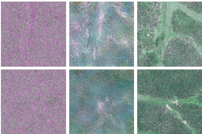
Figure 7. Qualitative examples illustrating the limitation of the SAR-to-optical translation model when the SAR input lacks clear structural information. Columns: (i) SAR input, (ii) model-generated optical image, and (iii) reference cloud-free Sentinel-2 image.
