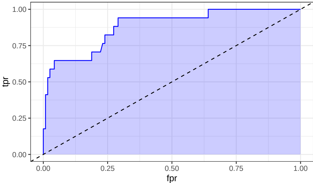
ROC Curve w/ AUC=0.883
