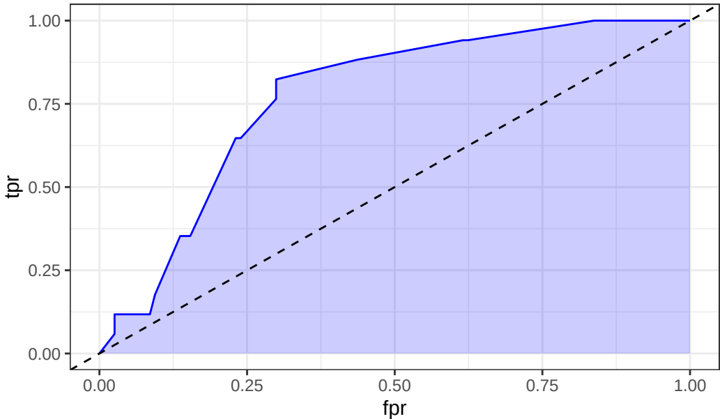
Model C: ROC Curve w/ AUC=0.771
