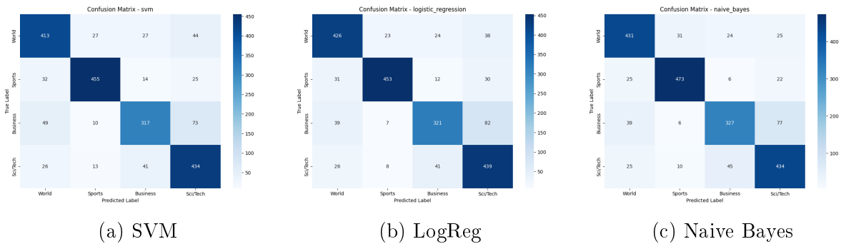
Figure 3: Confusion Matrices for Traditional Models
