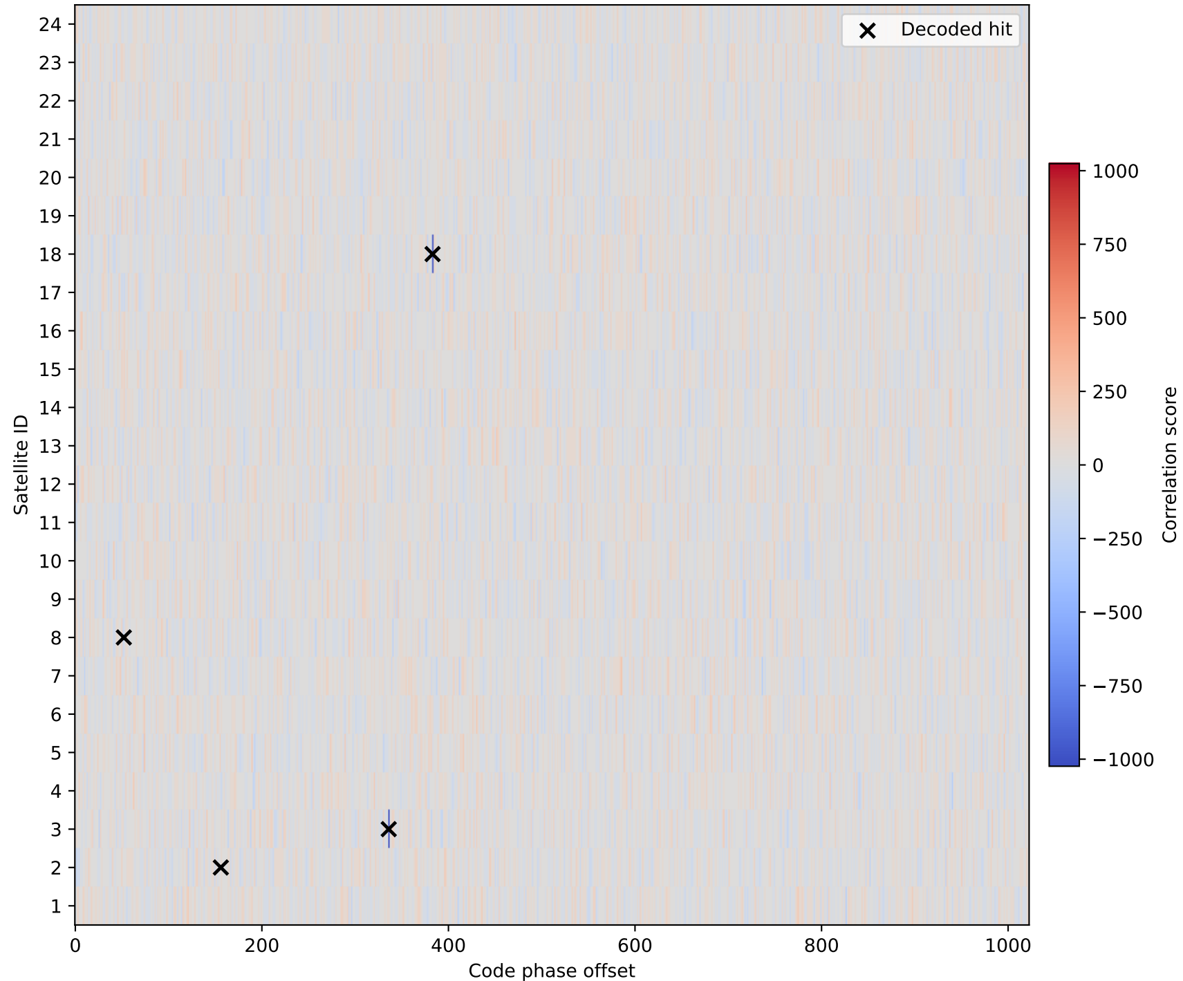
CDMA Correlation Landscape (satellite x code phase)
