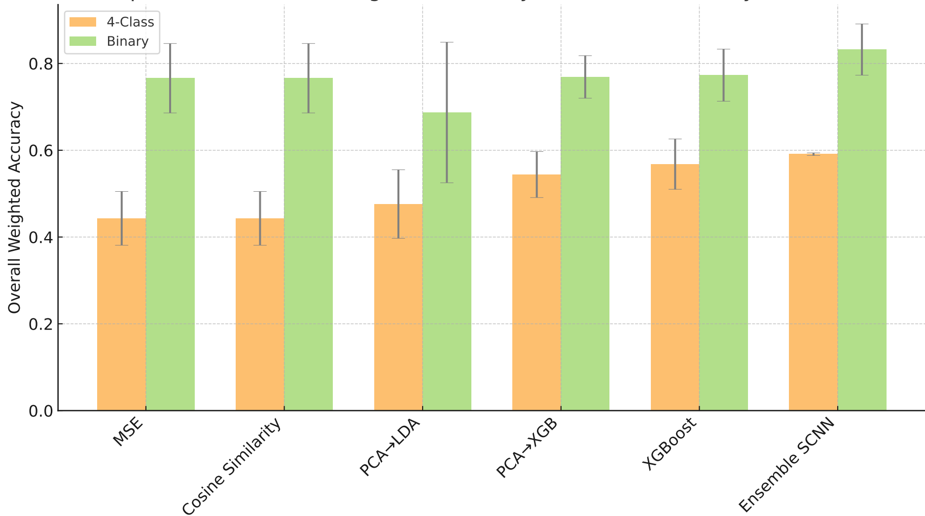
Comparison of Overall Weighted Accuracy for 4-Class vs Binary Classification
