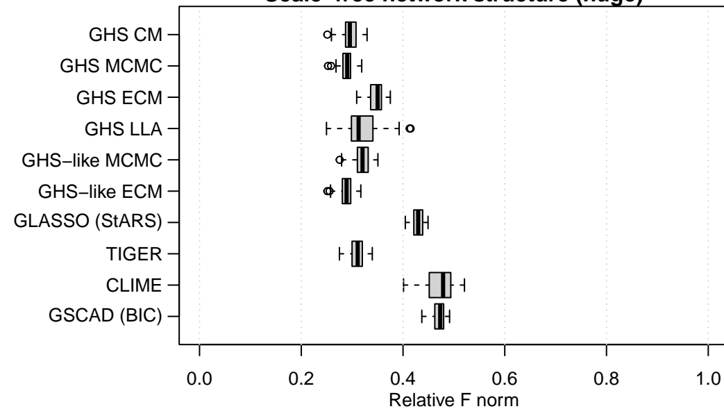
Scale-free network structure (huge)
