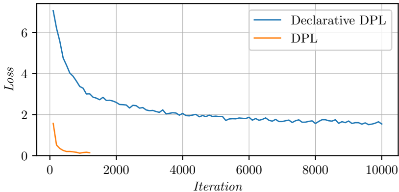
VAE Training Loss
