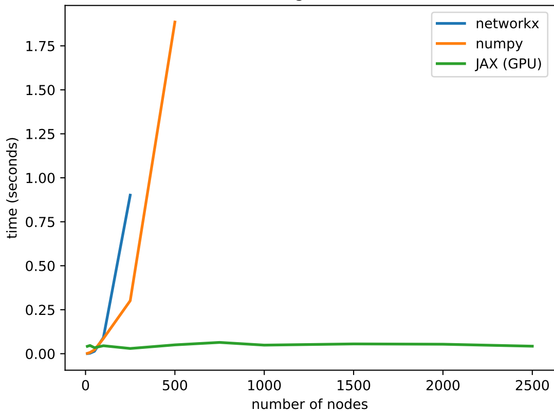
clustering coefficient
