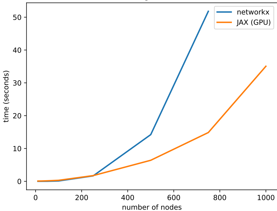
clustering coefficient
