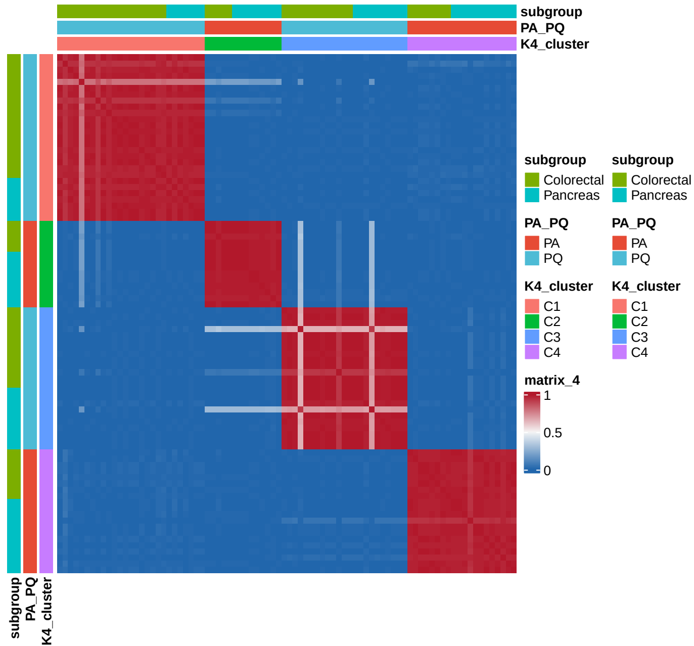
True K4 consensus matrix (84 samples)
