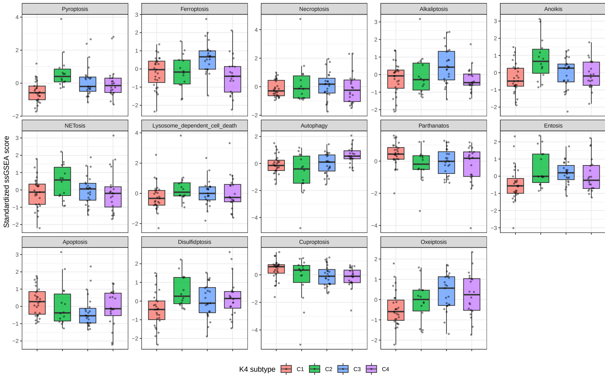
Programmed cell-death (PCD) scores across K4 subtypes
