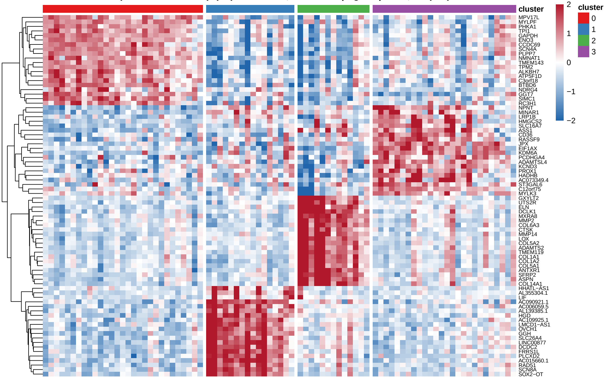
Top markers heatmap (Top 20/cluster; FDR<=0.1 |log2FC|>=0.5; zclip=2)
