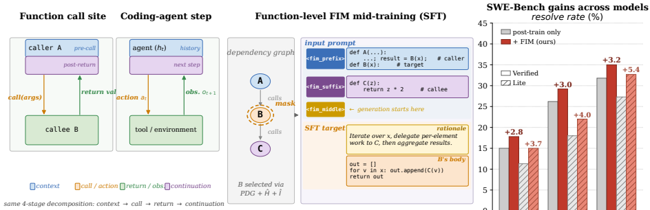
Figure 1: Left: A function call site and a single step of a coding agent are structurally similar , decomposing into the same four stages: context, call/action, return/observation, continuation. Middle: We exploit this analogy via function-aware FIM mid-training. A function B is selected from the program dependency graph using complexity ( \hat{H} ) and inferability ( \hat{I} ) scores; the model is then mid-trained to fill in B 's body together with a CoT rationale, given the surrounding file as an FIM-formatted prompt. Right: Mid-training yields consistent gains across both Qwen2.5-Coder-Instruct (7B, 14B) and Qwen3 (8B) on SWE-Bench-Verified (solid bars) and SWE-Bench-Lite (hatched bars).
