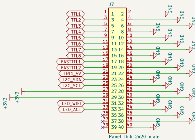
J7 – digital, at x = 90 mm on the bottom side
