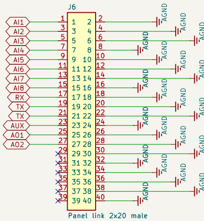
J6 – analog, at x = 12 mm on the bottom side
