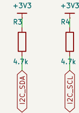
I2C 400 kHz pull–ups (OLED 0x3C + Qwiic J4 inside + the panel Qwiic)
