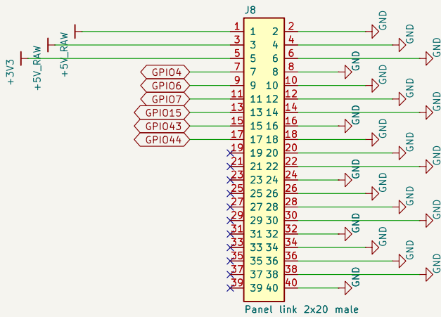
J8 – power + spares, at x = 168 mm on the bottom side
