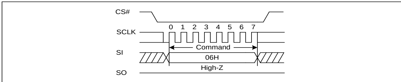
Figure2. Write Enable Sequence Diagram
