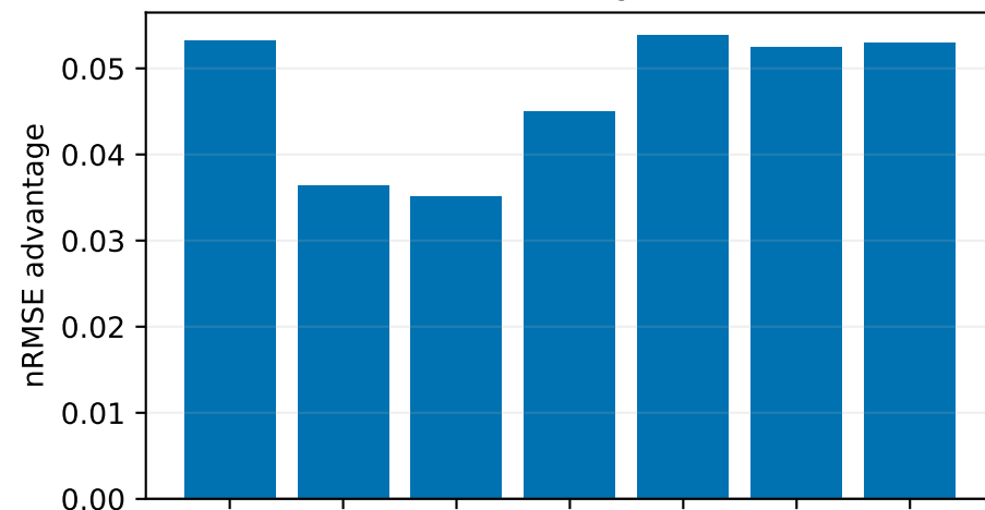
Linear interpolation vs TIMESAT double logistic (default)
