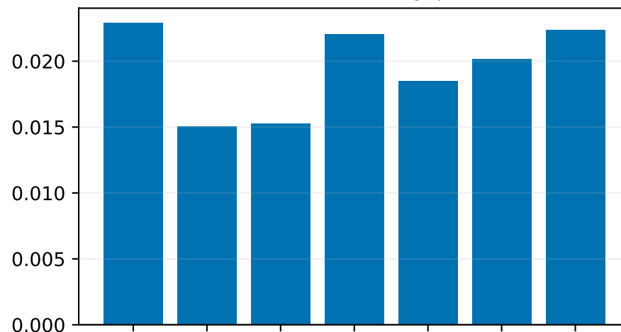
Linear interpolation vs TIMESAT smoothing spline
