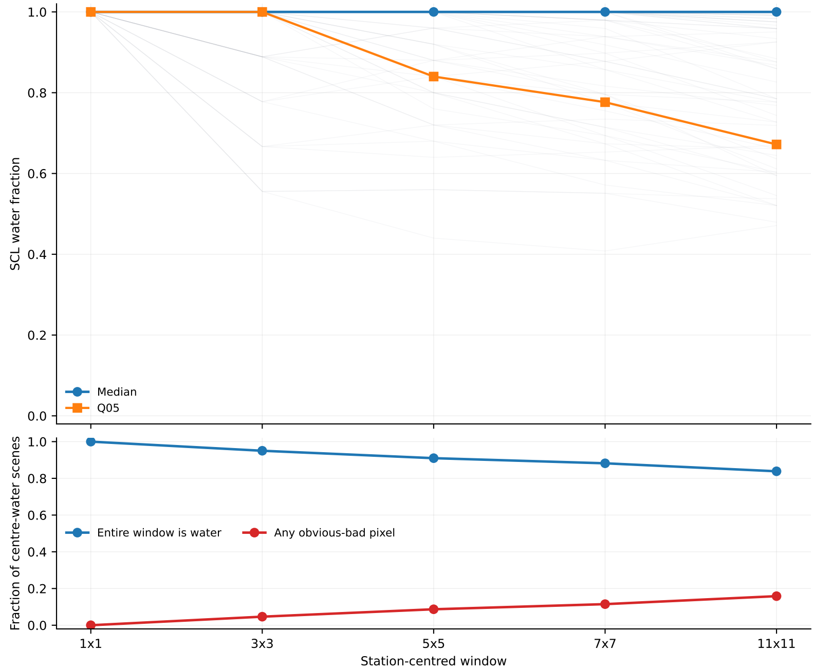
Paired spatial expansion for acquisitions with a water centre pixel
