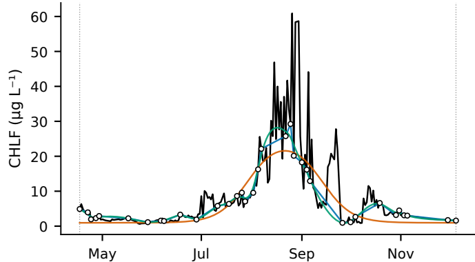
2021 (spline p_{\text{smooth}} = 100 )
