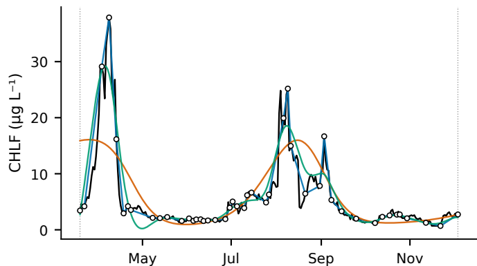
2023 (spline p_{\text{smooth}} = 10 )
