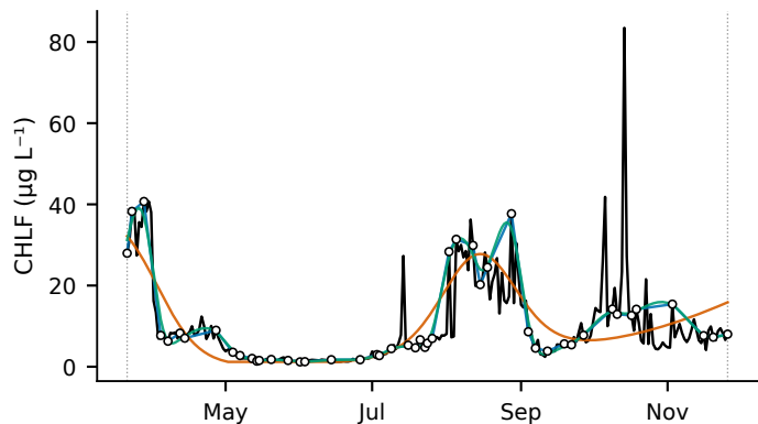
2025* (spline p_{\text{smooth}} = 10 )
