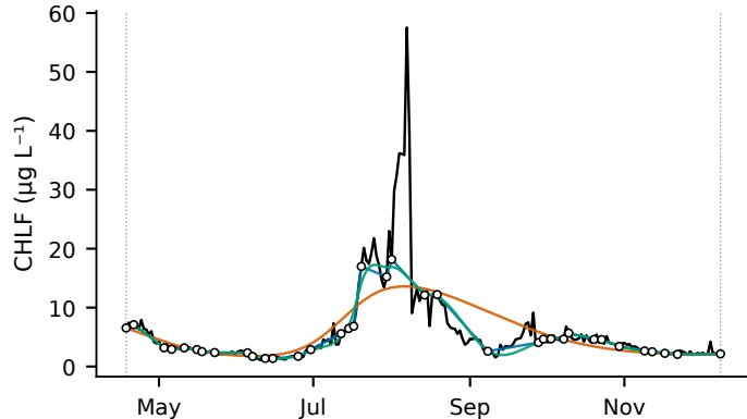
2024 (spline p_{\text{smooth}} = 3 )
