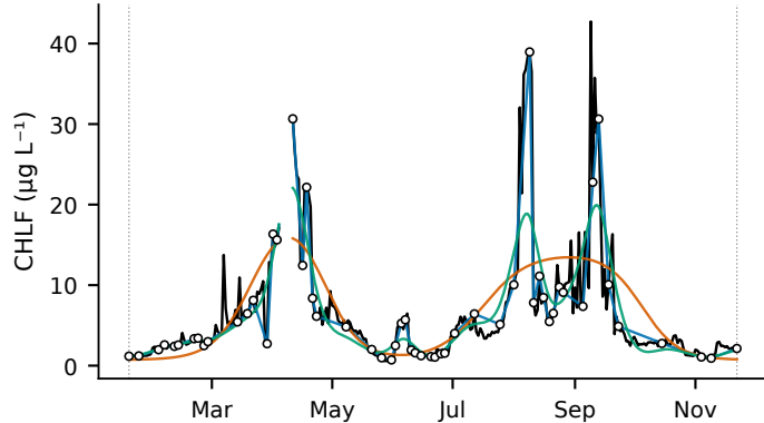
2022 (spline p_{\text{smooth}} = 10 )
