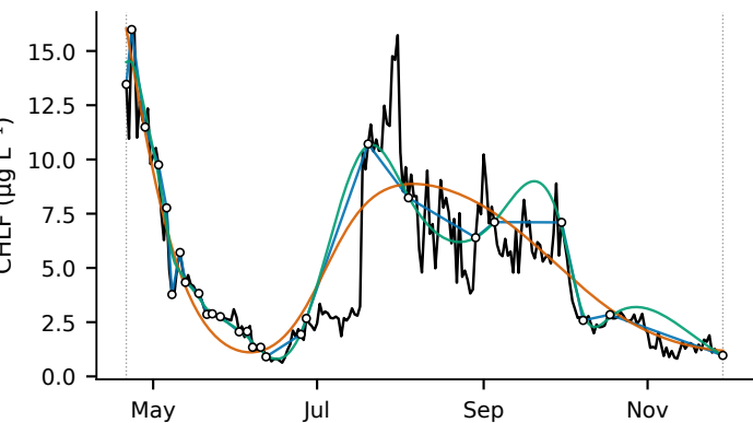
2025* (spline p_{\text{smooth}} = 10 )
