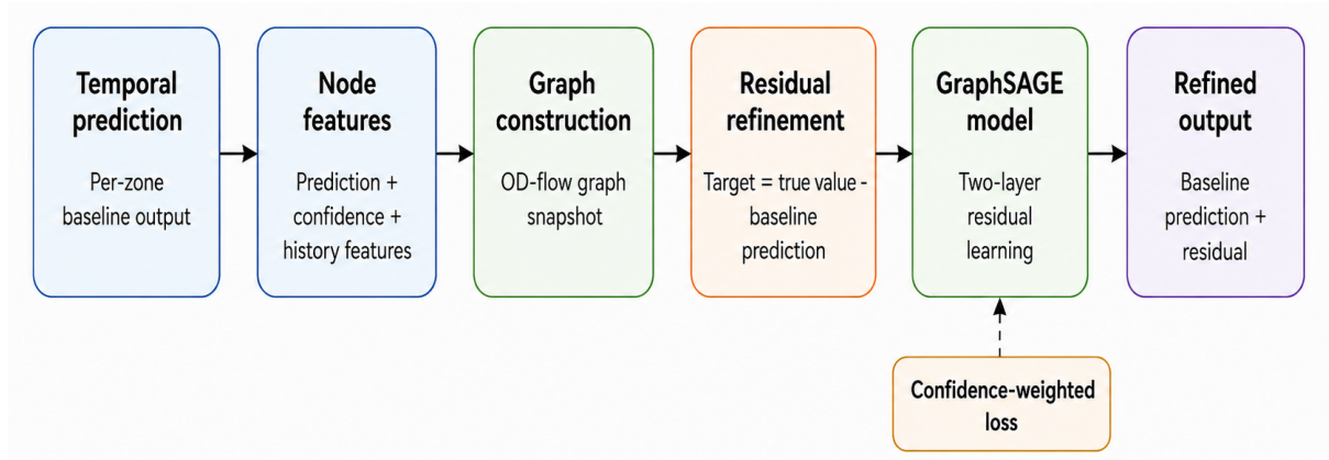
Figure 3.4: Graph-based residual refinement at each rolling step. The hourly taxi-zone graph is built from valid nodes, baseline predictions, confidence scores, and historical features, and a two-layer GraphSAGE model learns residual corrections that are added to the temporal baseline to obtain the final refined forecast. Confidence is injected through node-weighted loss rather than direct edge-weighted message passing.
