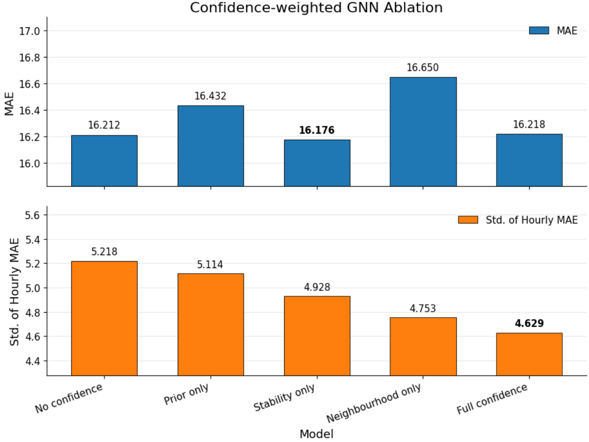
Figure 5.3: Confidence-weighted GNN ablation results, comparing unweighted graph refinement with prior-only, stability-only, neighbourhood-only, and full confidence weighting strategies.
