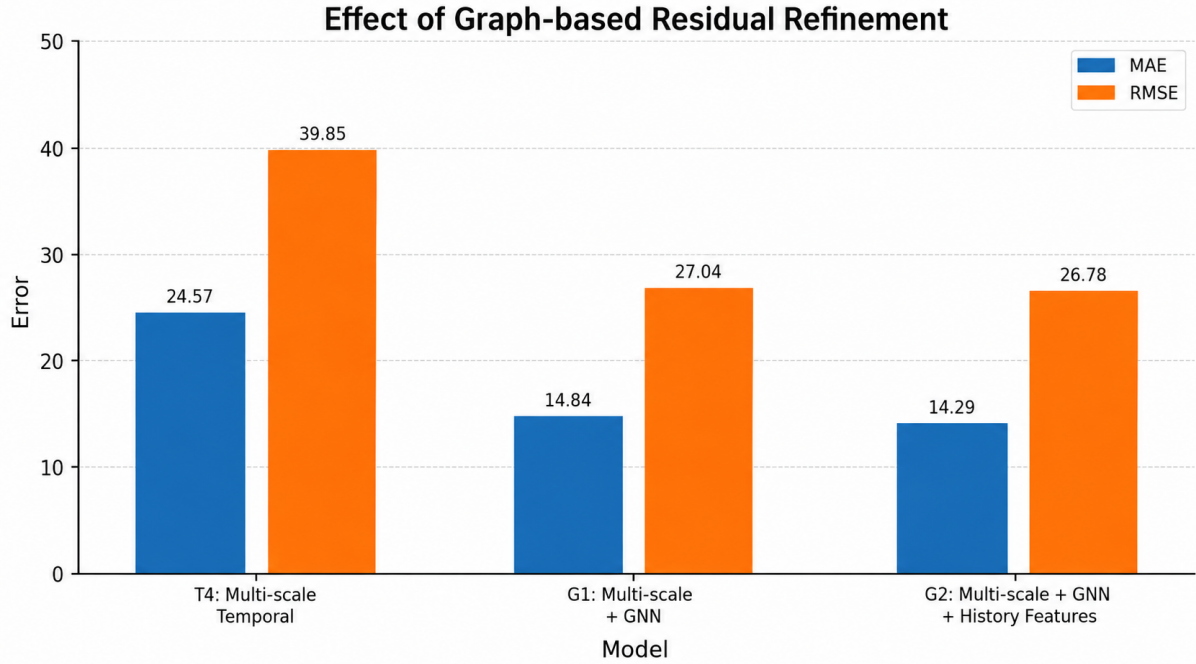
Figure 5.2: Effect of GraphSAGE-based residual refinement on multi-scale temporal predictions, comparing the temporal-only model with graph-refined variants with and without historical mean features.
