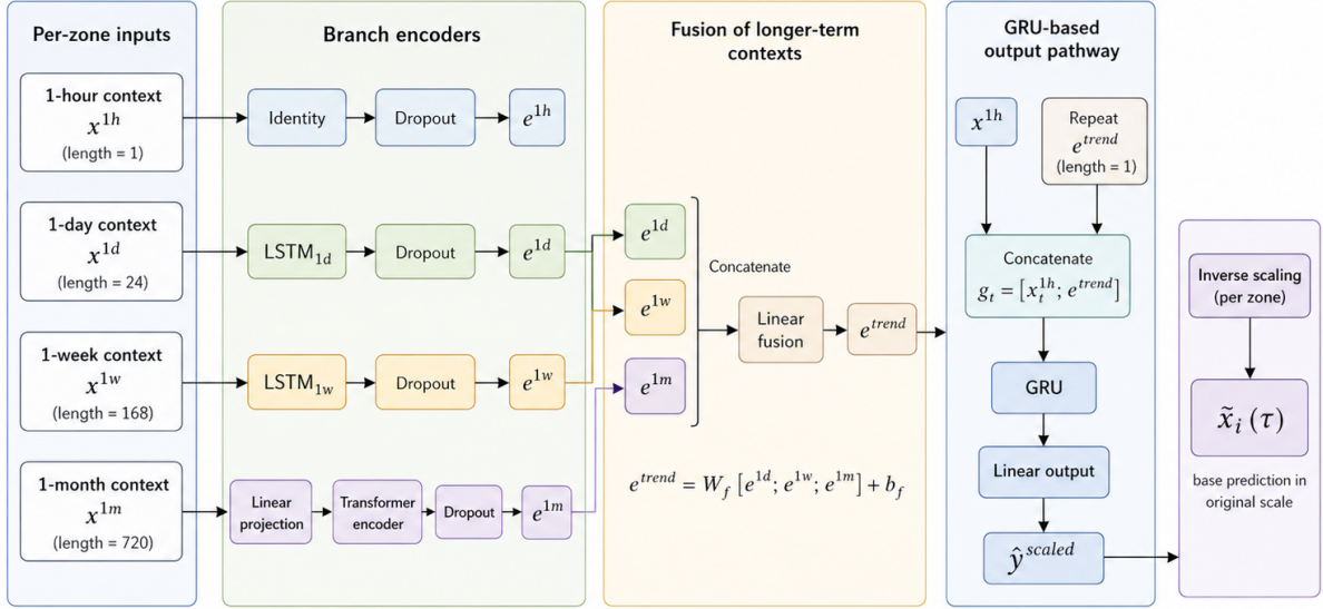
Figure 3.2: Stage-one temporal forecasting pipeline for each taxi zone. Multi-scale inputs from 1 hour, 1 day, 1 week, and 1 month are encoded by branch-specific modules, fused into a longer-term trend representation, and combined with the short-term signal in a GRU-based output pathway to generate the next-hour demand prediction in the original scale.
