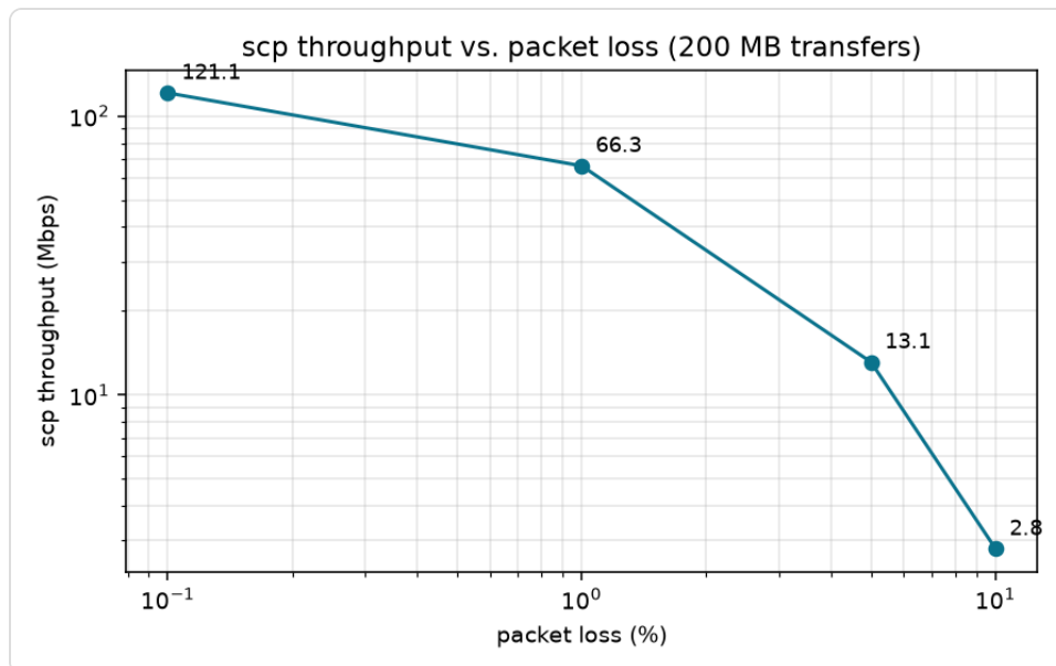
Fig. 1 — scp throughput vs. packet loss (200 MB transfers).
