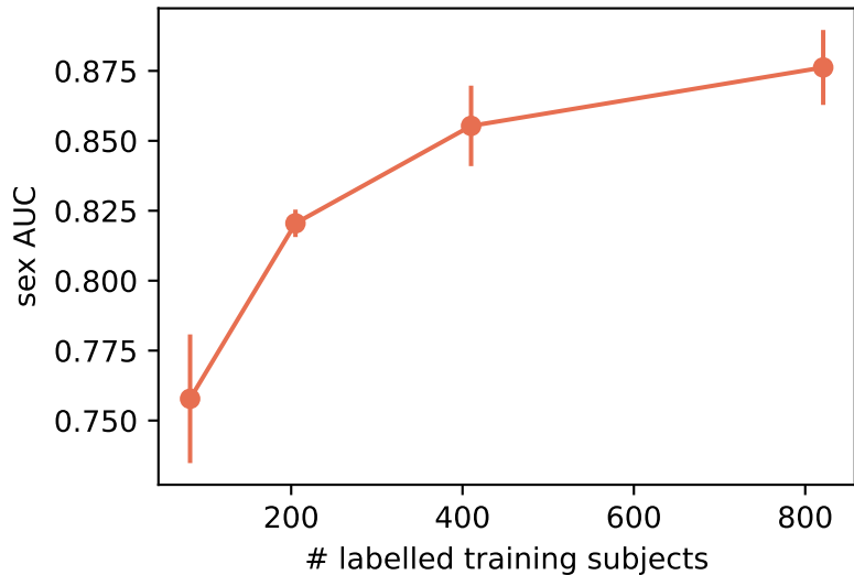
Data efficiency
