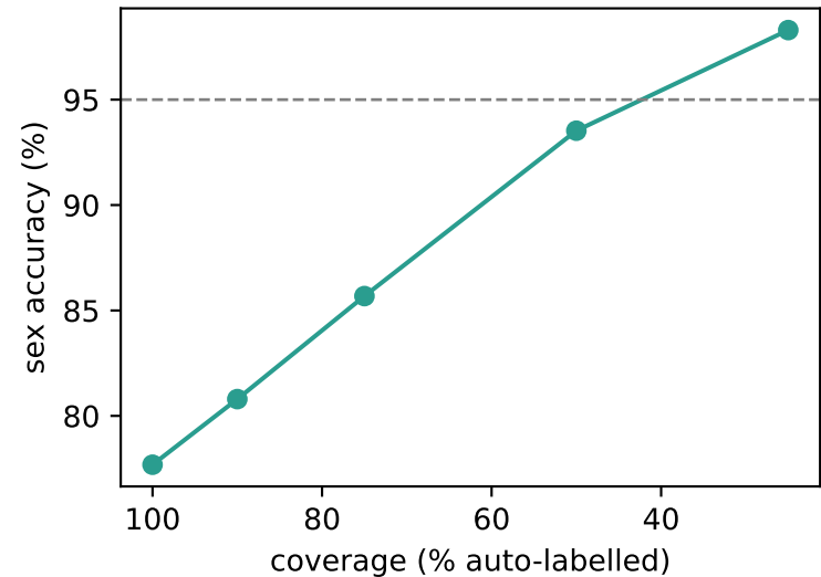
Selective auto-labelling
