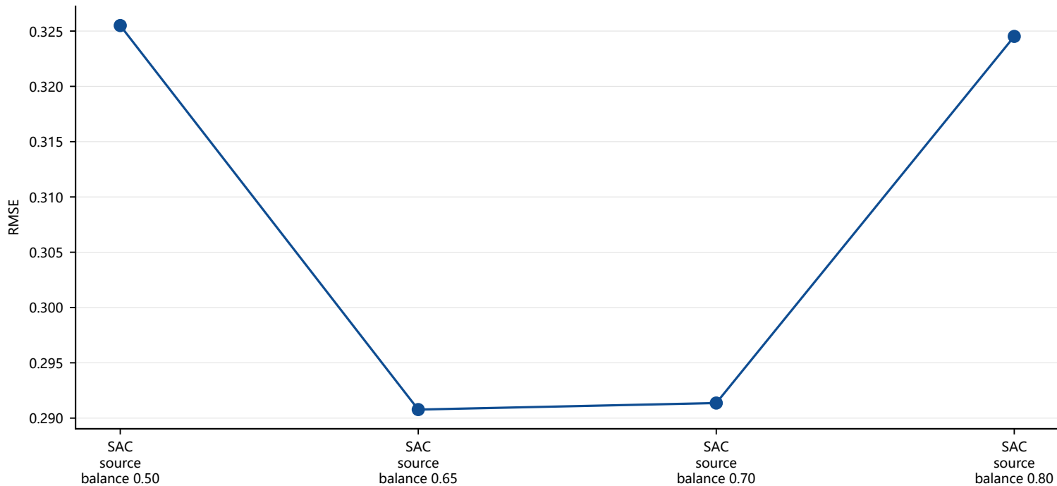
参数敏感性: second_src_balance
