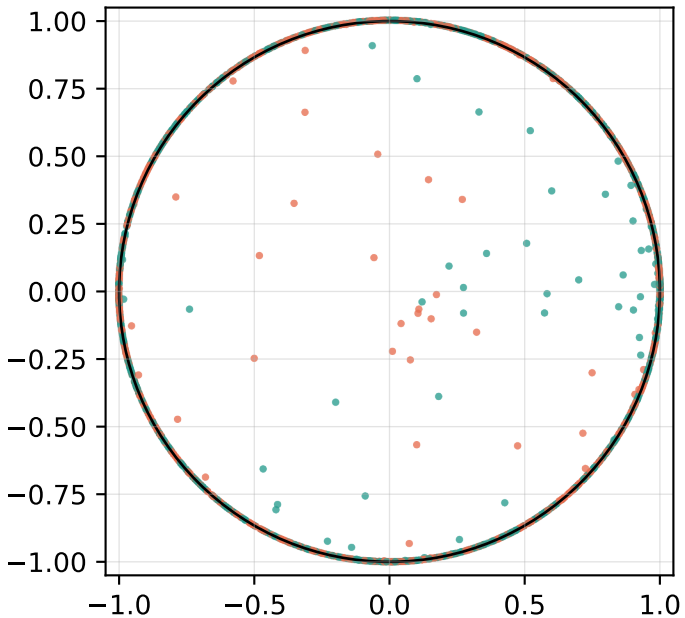
Vanilla Embeddings
