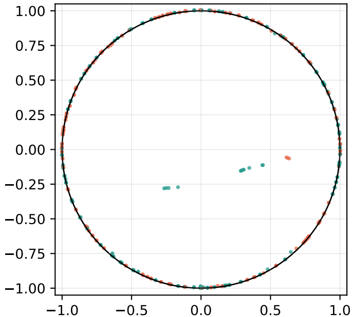
Trained Embeddings
