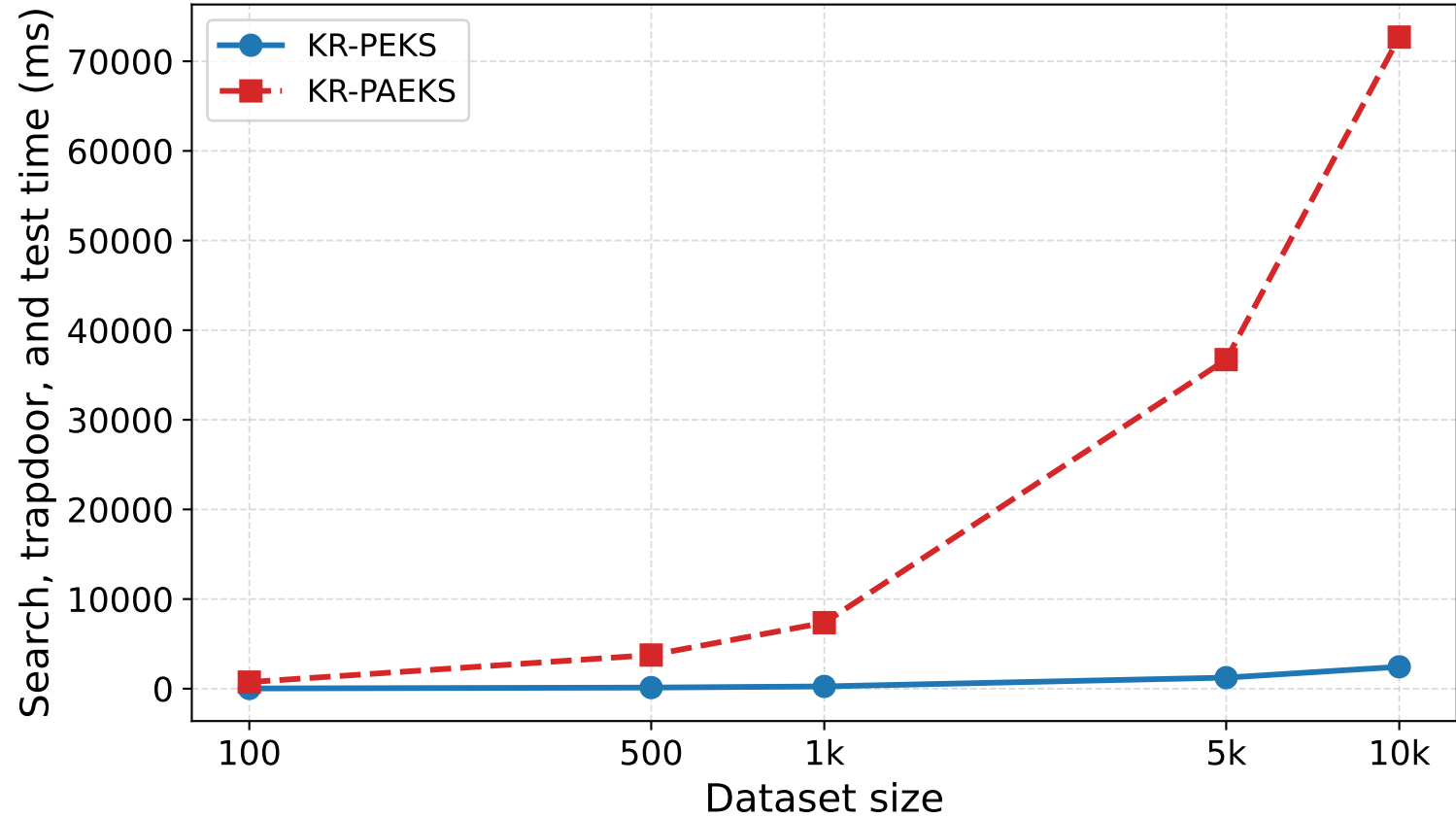
Dataset Size vs. Search Time
