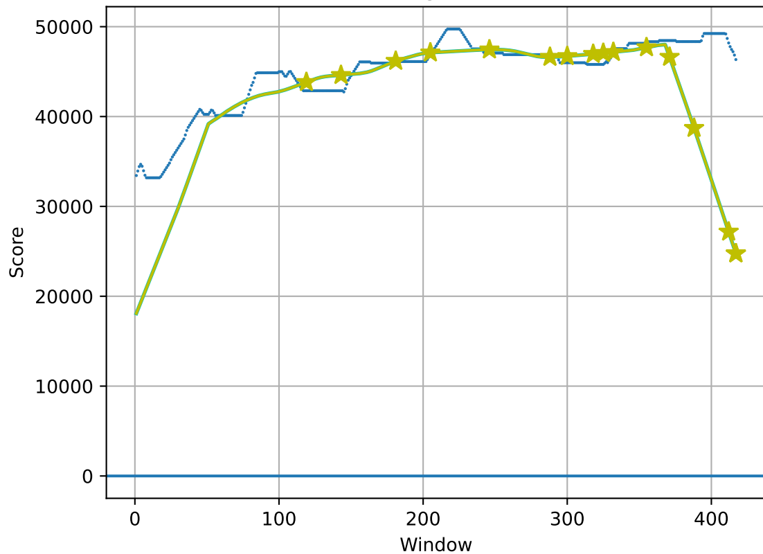
Viral region calls
