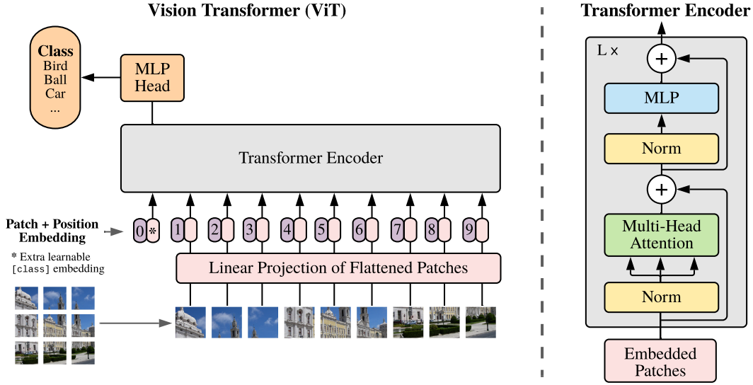
Figure 1.6: Vision Transformer Overview.
