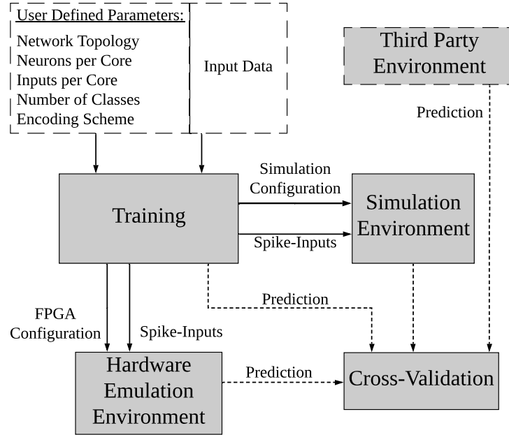
Figure 1.5: Training, Testing, and Emulation environment of offered by RANC.
