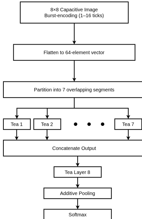
Figure 2.3: RANC-based SNN Model architecture
