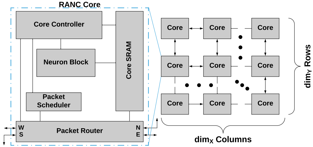
Figure 1.4: High level architectural overview of RANC[8] components.
