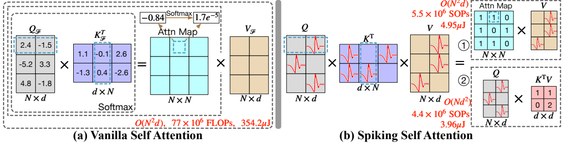
Figure 1.8: Illustration of vanilla self-attention (VSA)[26] and Spiking Self Attention (SSA)[29]
