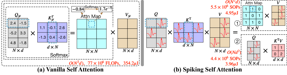
Figure 2.8: Illustration of vanilla self-attention (VSA)[25] and Spiking Self Attention (SSA)[28]
