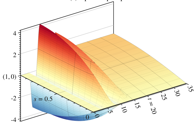
(a) Open-loop response
