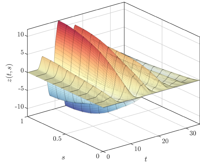
(a) Open-loop response
