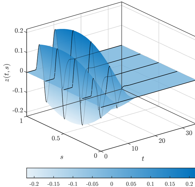
(b) Closed-loop response
