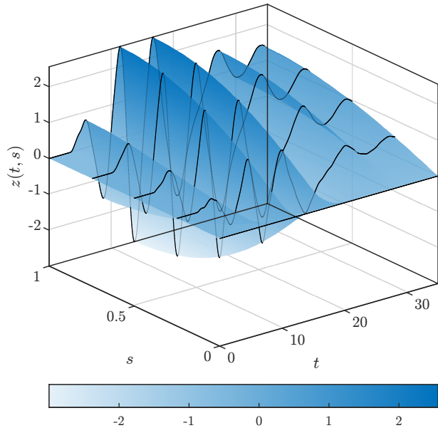
(a) Open-loop response
