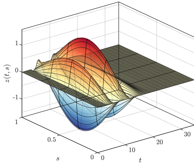
(b) Closed-loop response
