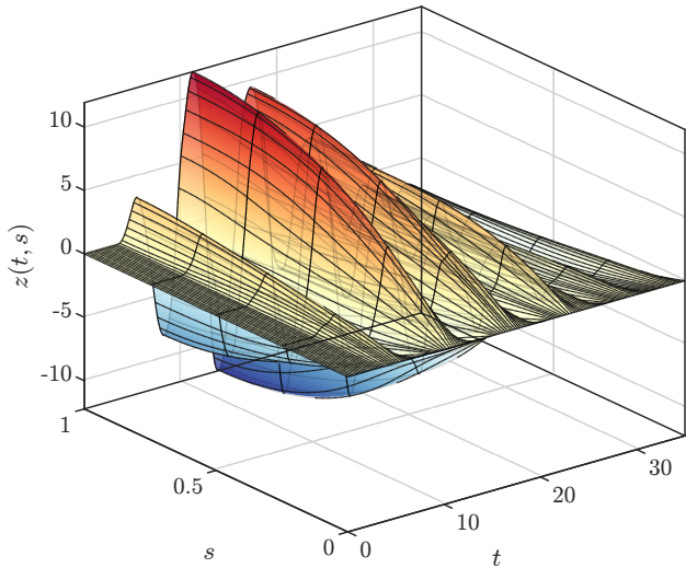
(a) Open-loop response
