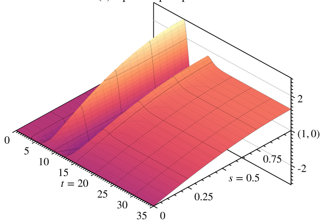
(a) Open-loop response
