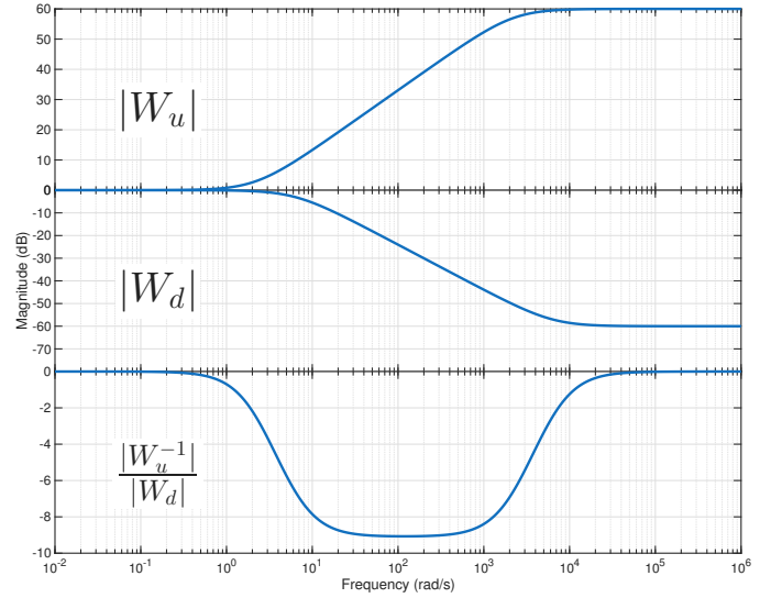
Fig. 3. Bode magnitude plots of the input and disturbance weighting filters, W_u and W_d , together with the combined inverse weighting W_u^{-1}W_d^{-1} . These weights are used to encode the desired frequency-dependent characteristics of the control input and disturbance in the weighted boundary control synthesis.
