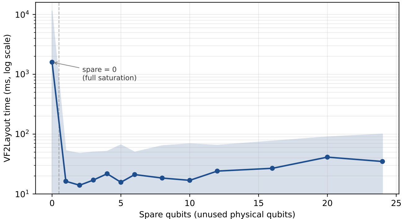
Occupancy cliff: VF2Layout on a 6 \times 7 grid, dense-pair circuits
