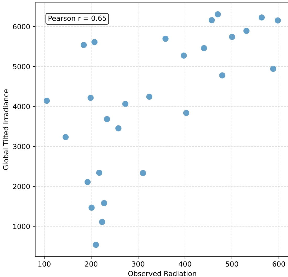
Observed Radiation vs Global Tilted Irradiance
