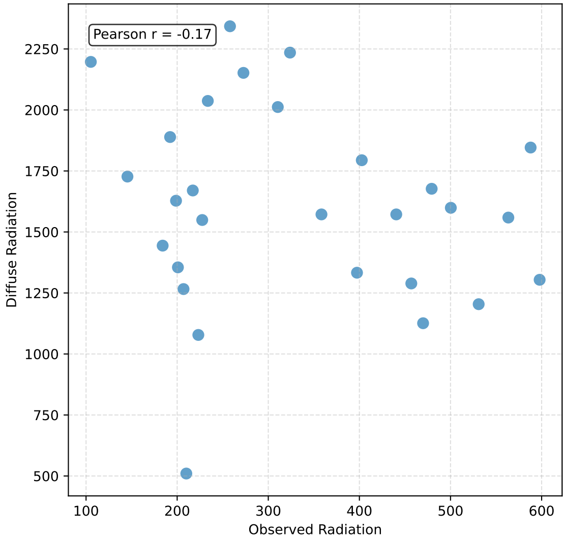
Observed Radiation vs Diffuse Radiation
