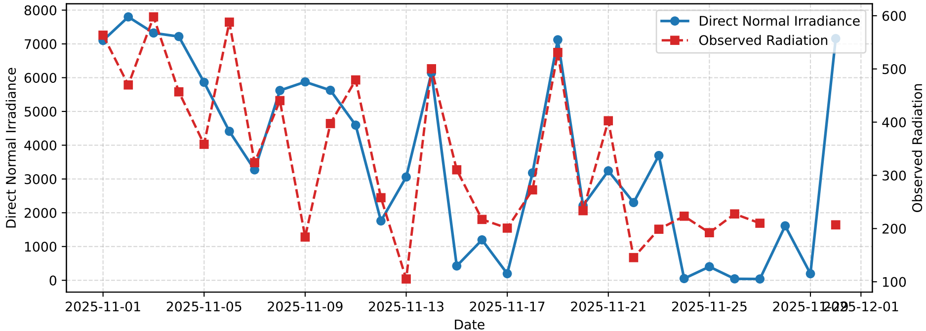
Daily Direct Normal Irradiance vs Time
