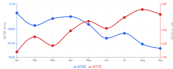
MTBF and MTTR Trends Over Time
