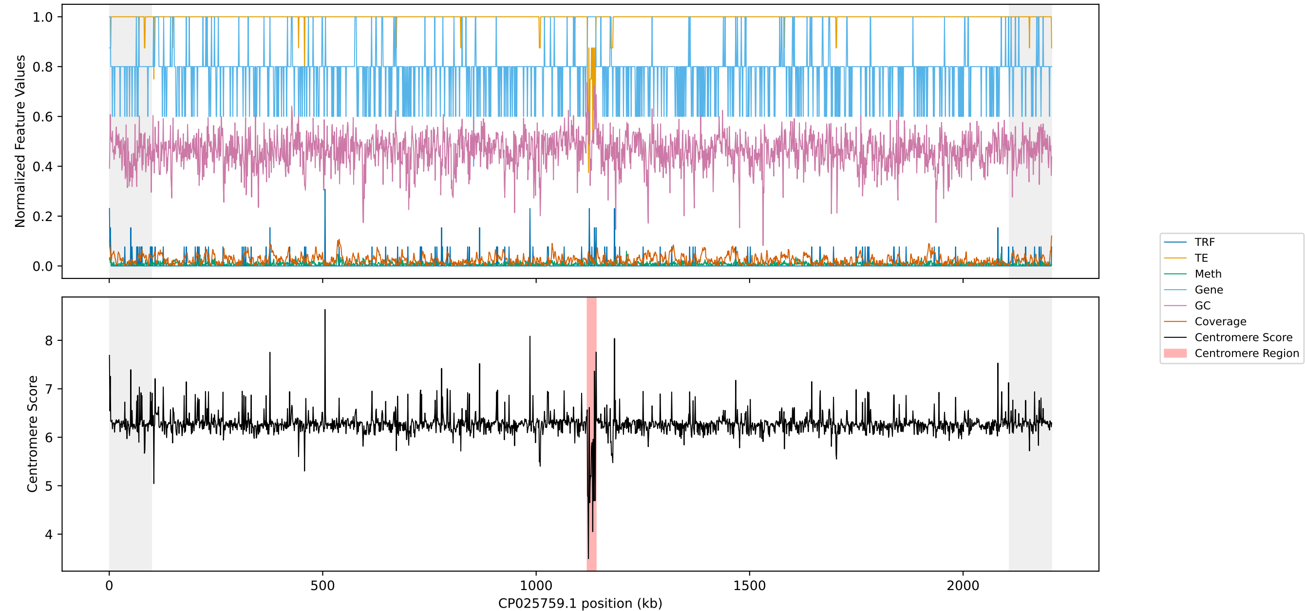
CP025759.1 - Features & Centromere Score
