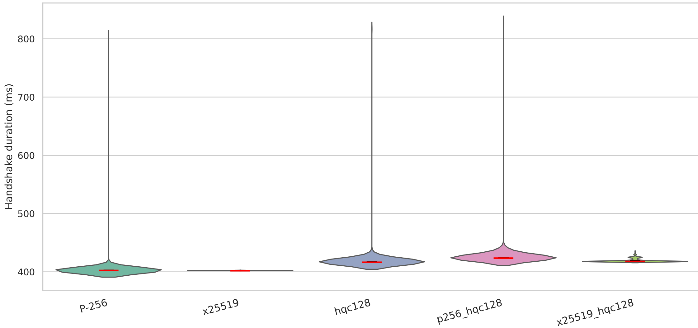
Handshake duration on QUIC with ed25519 signature algorithm — Degraded (200ms/10%)
