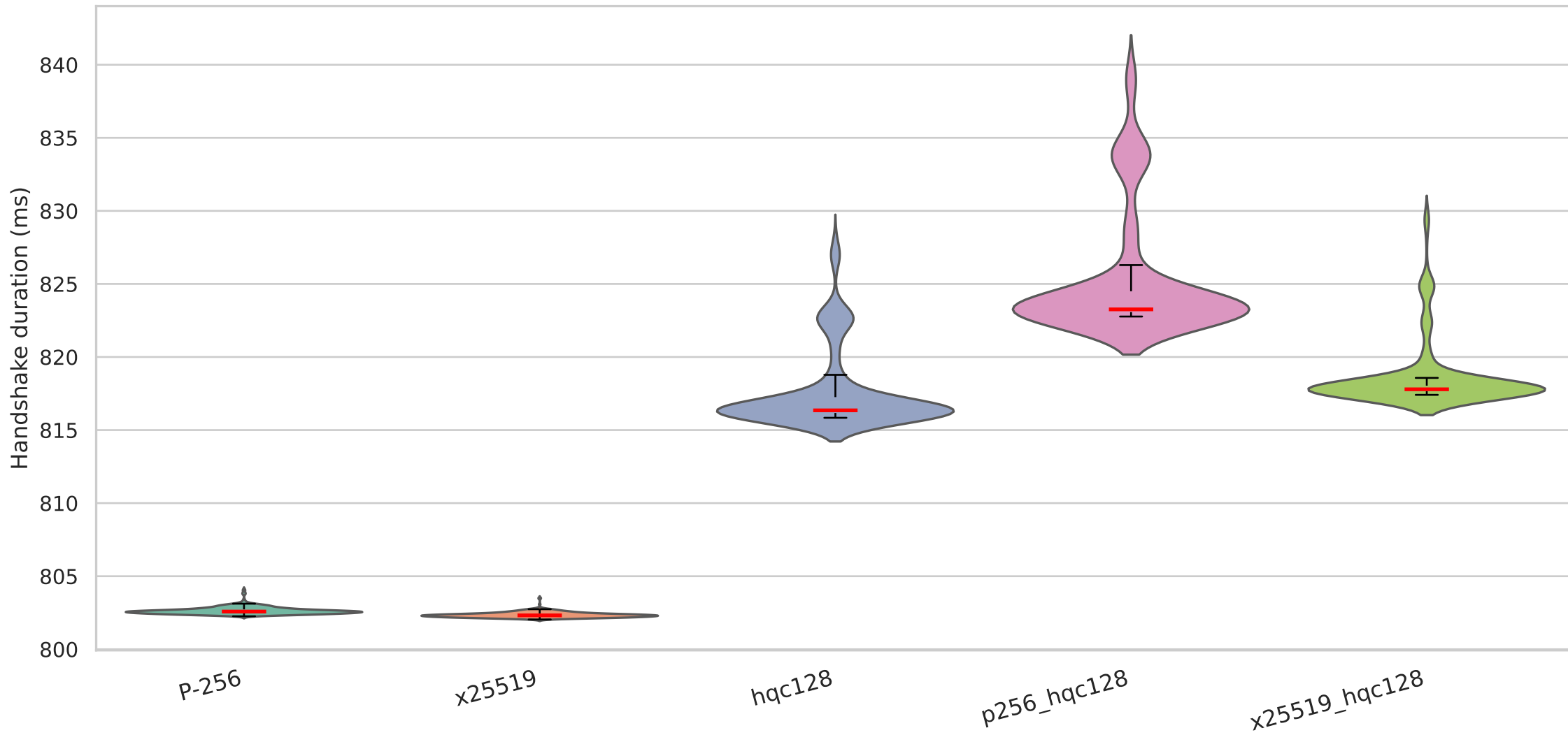
Handshake duration on QUIC with mldsa44 signature algorithm — Backbone (200ms/4%)
