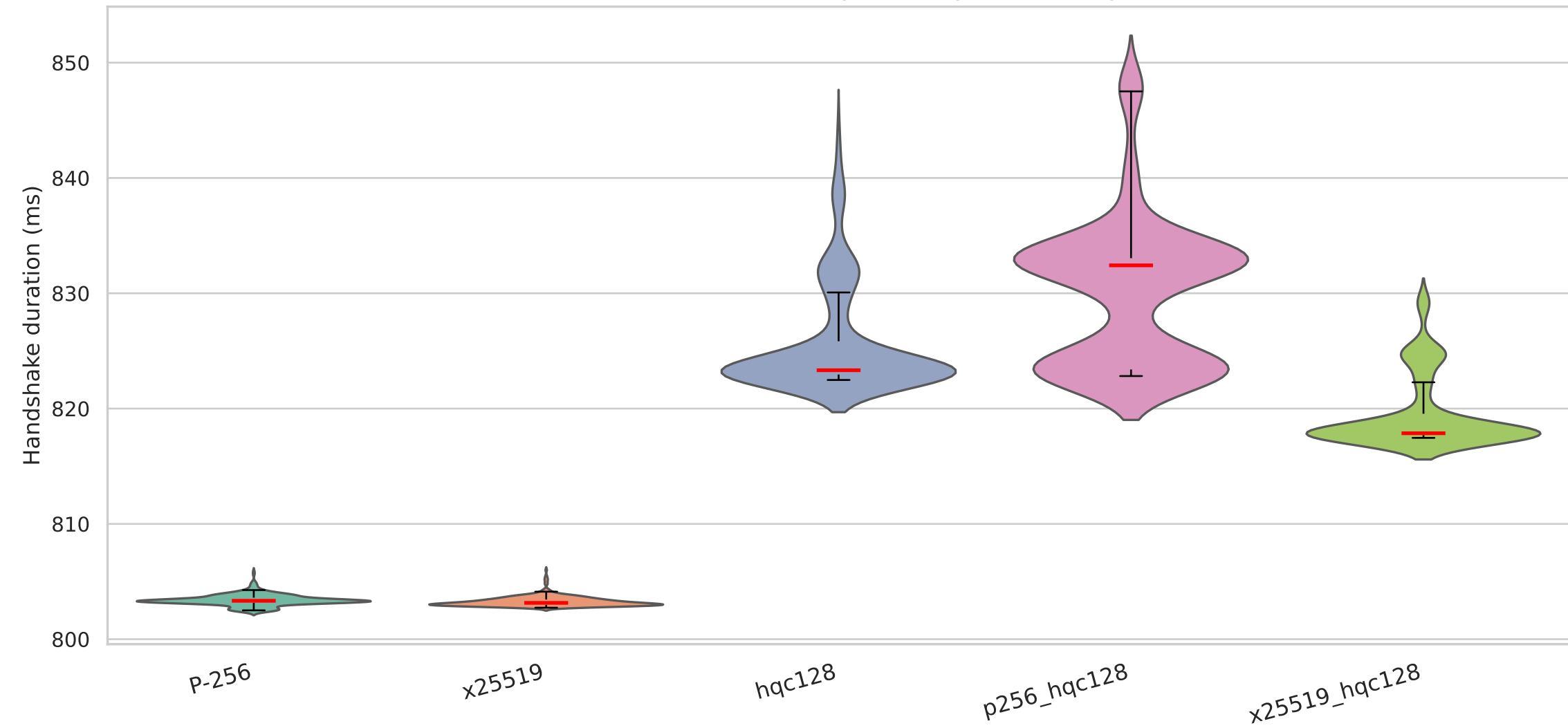
Handshake duration on QUIC with mldsa44 signature algorithm — Degraded (200ms/10%)
